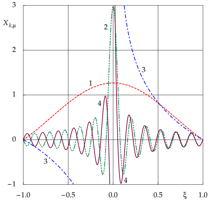
Fig. 5.1: The functions X_{k,\mu}(x) (5.2) (curve 1: k = 1 , \mu = 1 ; curve 2: k = 1 , \mu = 12 ; curve 3: k = 2 , \mu = 1 ; curve 4: k = 2 , \mu = 12 ; both branches of curves 3, 4 are anti-symmetric). The transformation |\xi| = |x|^{\frac{2-\alpha}{2}} stretches the neighborhood of the degeneracy point, acting like a magnifying glass.
